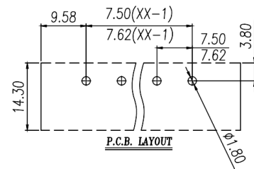
PCB开孔图 PCB Opening diagram
