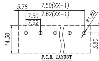
PCB开孔图 PCB Opening diagram
