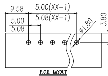
PCB开孔图 PCB Opening diagram
