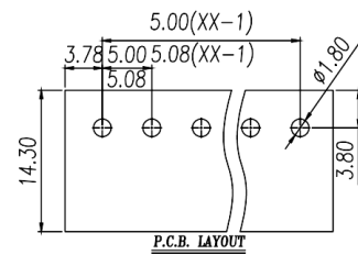
PCB开孔图 PCB Opening diagram
