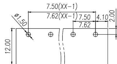
PCB开孔图 PCB Opening diagram
