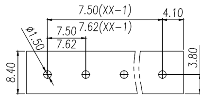
PCB开孔图 PCB Opening diagram
