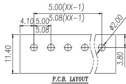
PCB开孔图 PCB Opening diagram
