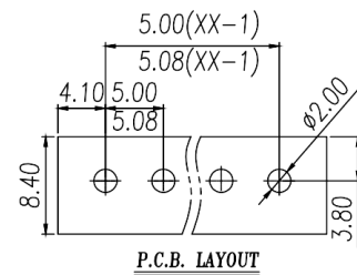
PCB开孔图 PCB Opening diagram
