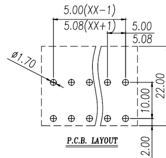
PCB开孔图 PCB Opening diagram
