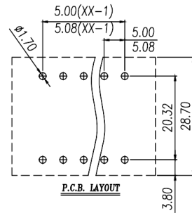
PCB开孔图 PCB Opening diagram
