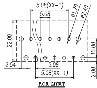
PCB开孔图 PCB Opening diagram
